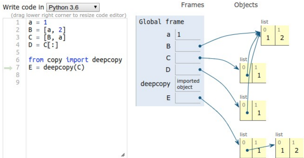
Abb. 80: deepcopy
